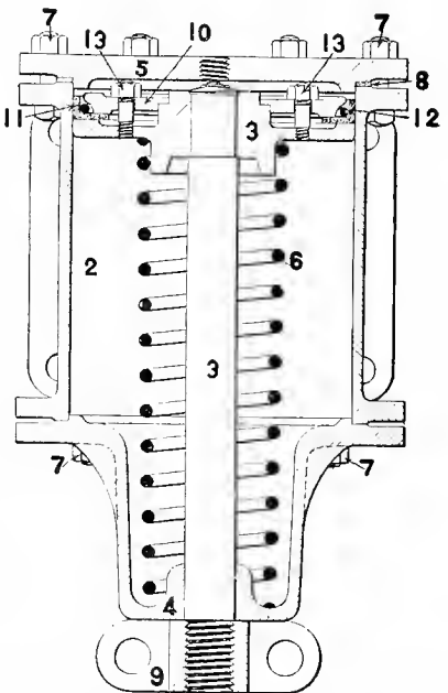
Fig. 1748. Push Down Driver-brake Cylinder.
